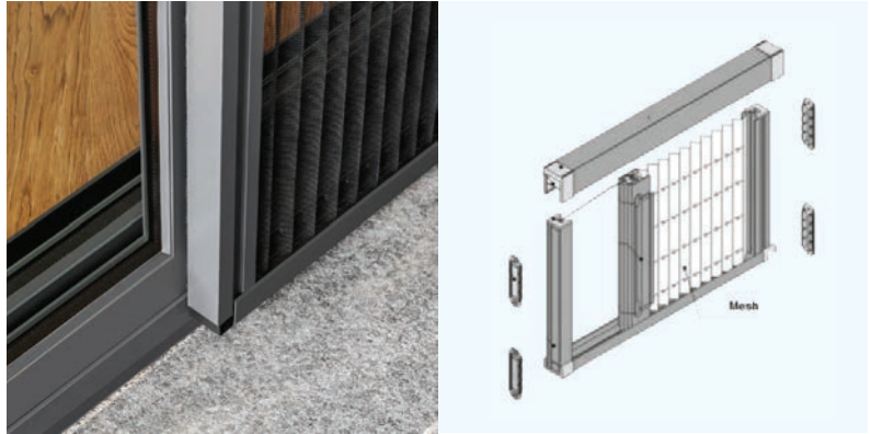
Face-fitted Byron system on a three panel glass sliding door.
