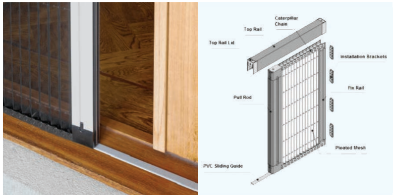
Airlie very low profile bottom track and mesh chain. Requires suitable surfaces for fitting.
